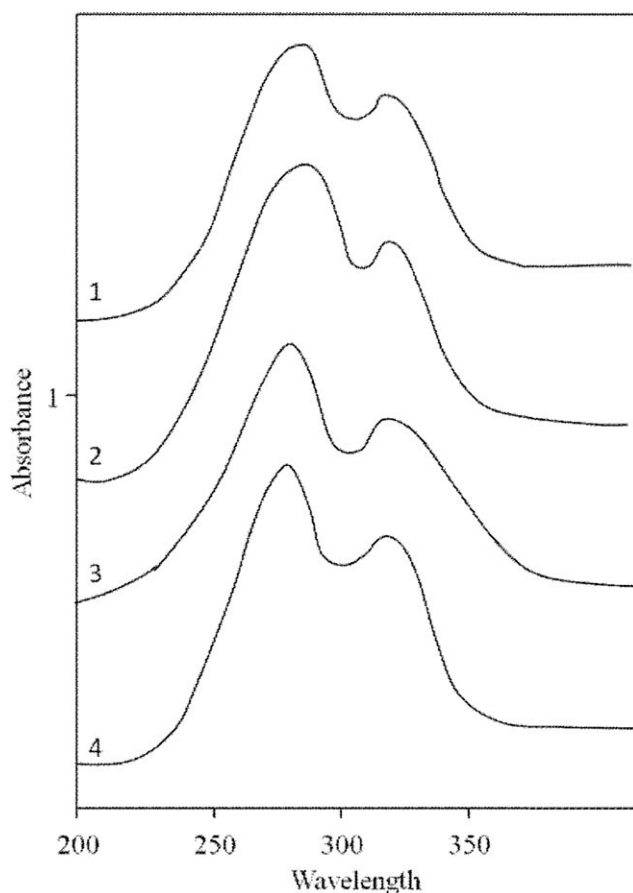
Figure 1 Electronic spectra of terpolymers: (1) 2,4-DHPOF-I (2) 2,4-DHPOF-II (3) 2,4-DHPOF-III (4) 2,4-DHPOF-IV.
